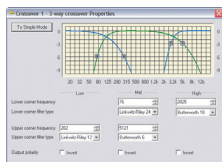
Crossover: 2-Way or 3-Way
